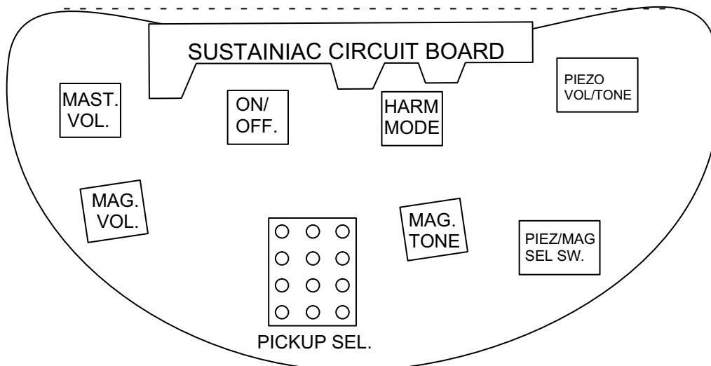
Electronics cavity showing location of Sustaiac circuit board and Sustaiac control switches
