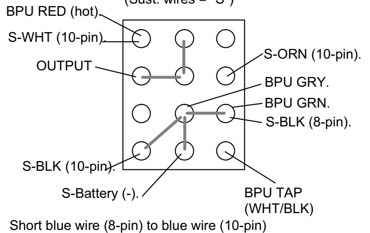
PICKUP SEL. SW DETAIL SHOWING SUST. INSTALLTION (Sust. wires = "S")
